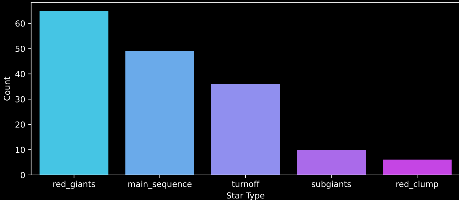
APOGEE DR17 Field: [286-25-O_TESS] Count plot of Star Type
