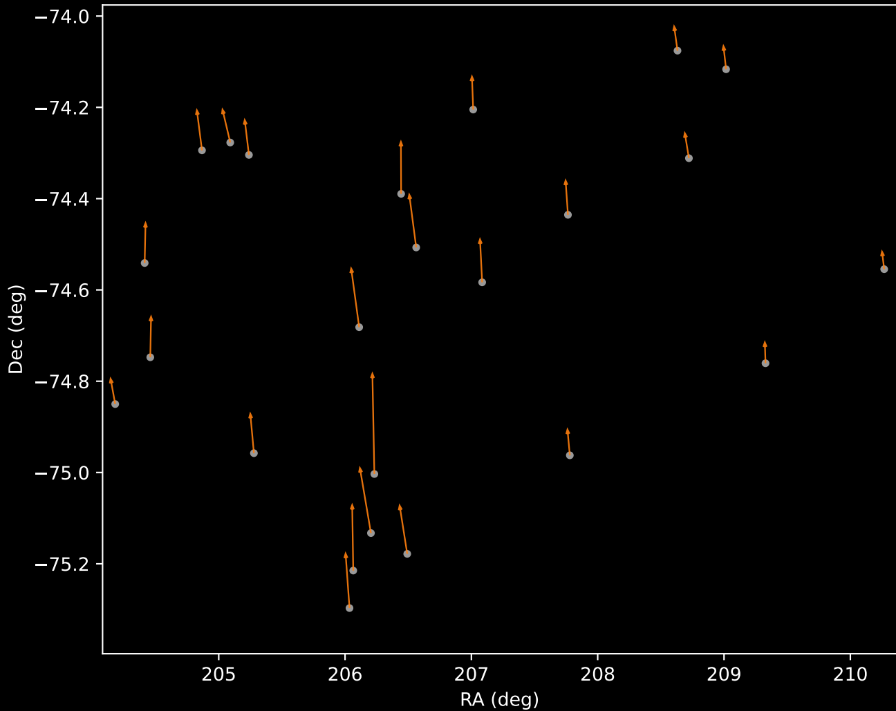
APOGEE DR17 Cluster 2 Proper Motion Vectors (n=24)
