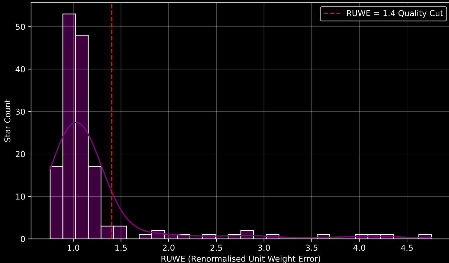
GAPOGEE DR17 Field [286-25-O_TESS] RUWE Distribution (n= 156)
