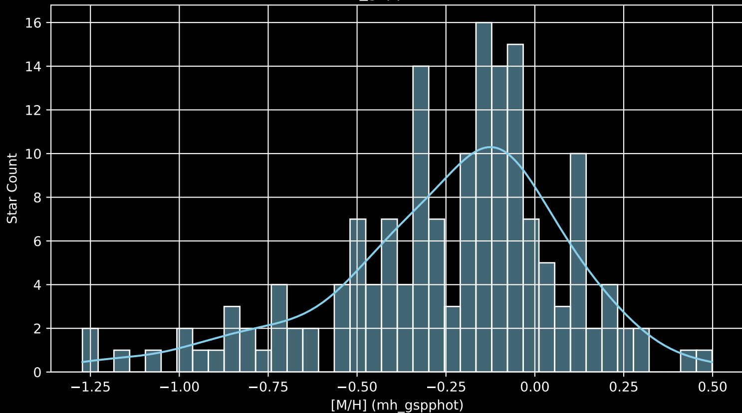
APOGEE DR17 Field: [286-25-O_TESS [M/H] (mh_gspphot) (n= 164)
