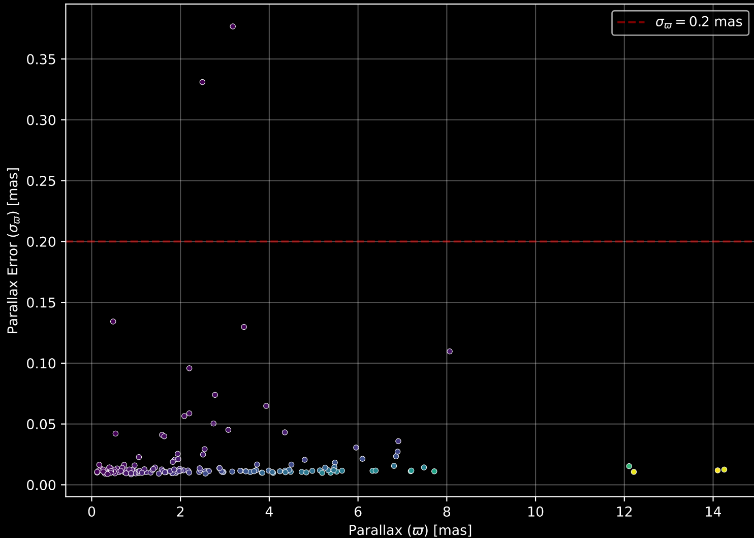
APOGEE DR17 Field: [286-25-O_TESS] Parallax Quality (n= 166)
