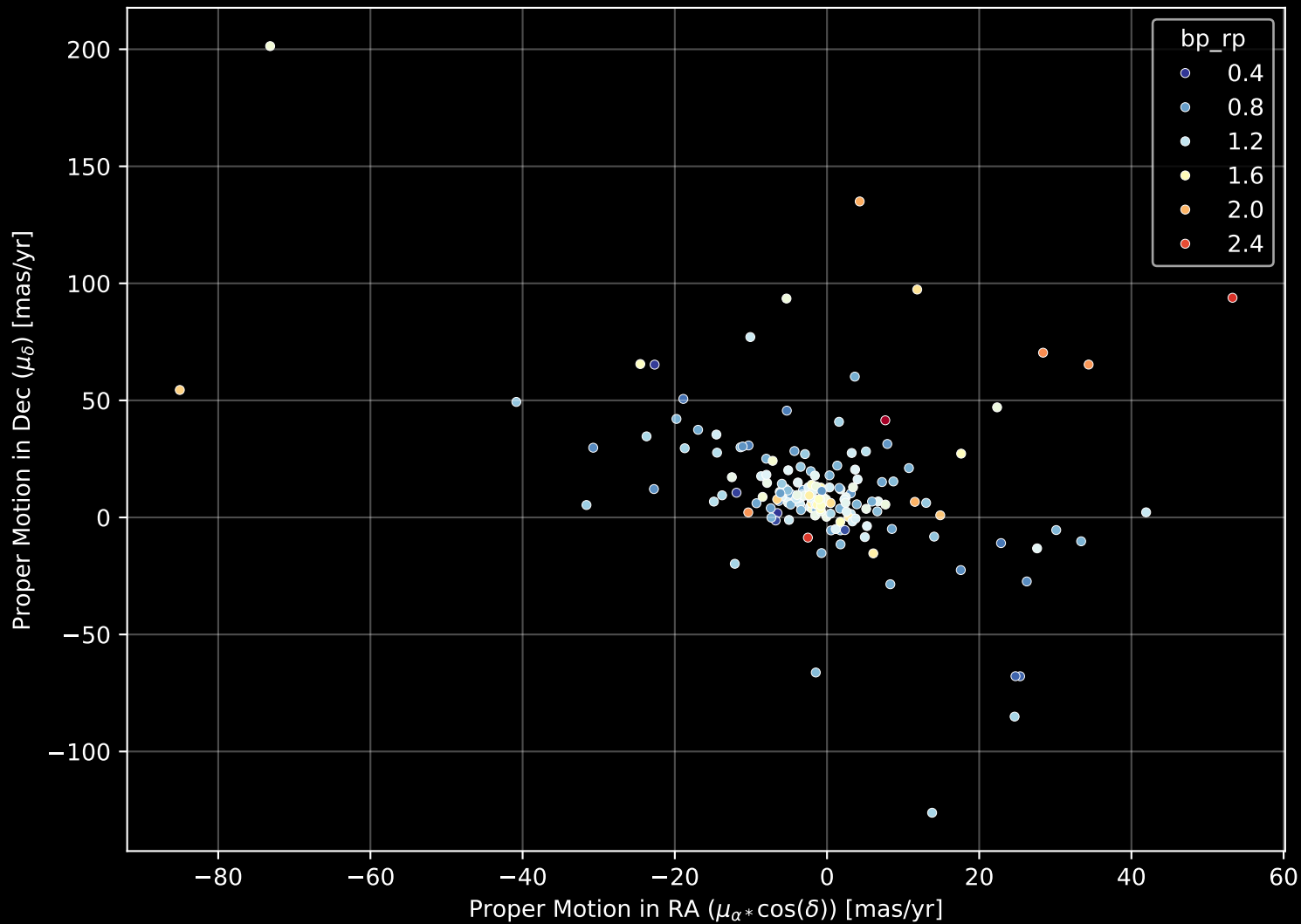
APOGEE DR17 Field: [286-25-O_TESS] Proper Motion Diagram (n= 166)
